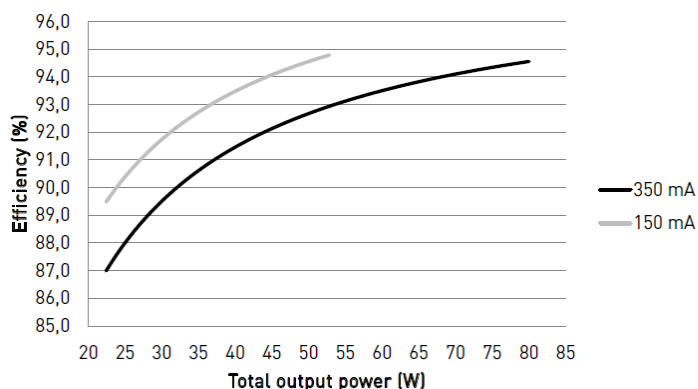
Typical efficiency
