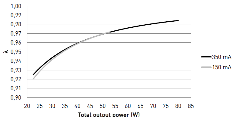
Typical power factor
