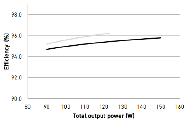
Typical efficiency
