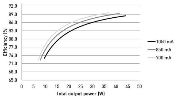
Typical efficiency
